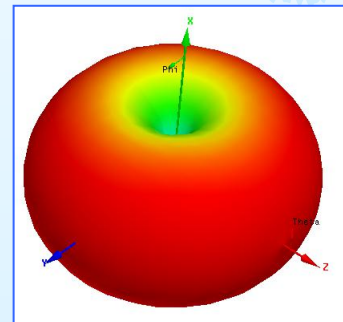
2.44GHz
