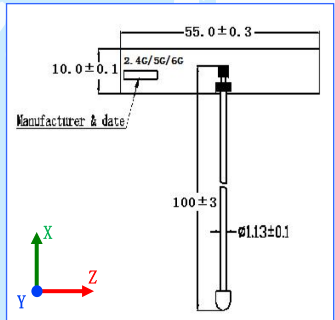
Dimensions (Unit: mm)
