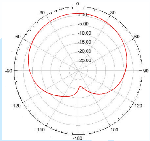
E-面@1616MHz
