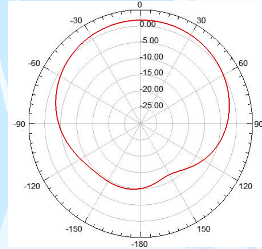
E-面@1616MHz
