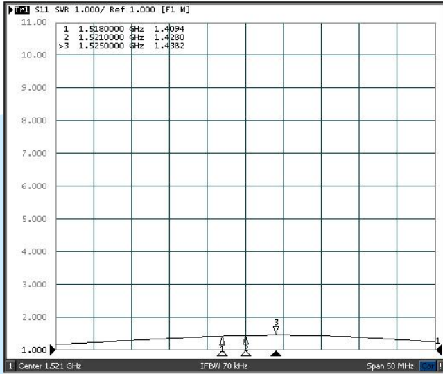
VSWR (1518~1525MHz)
