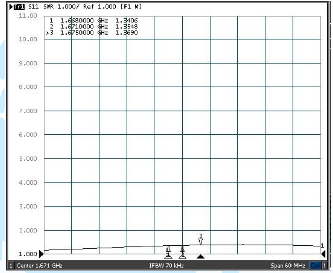
VSWR (1668~1675MHz)
